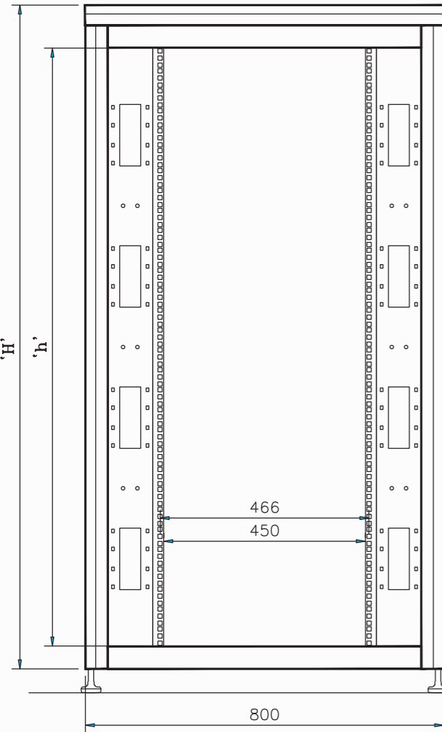
FRONT VIEW
